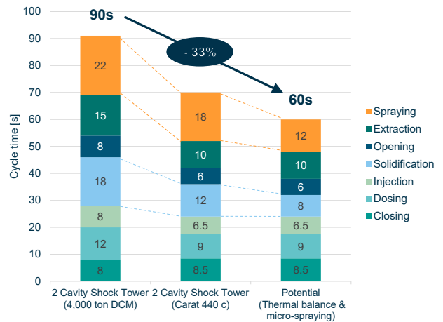
Figure 4: How better thermal management can reduce cycle times by up to a third
